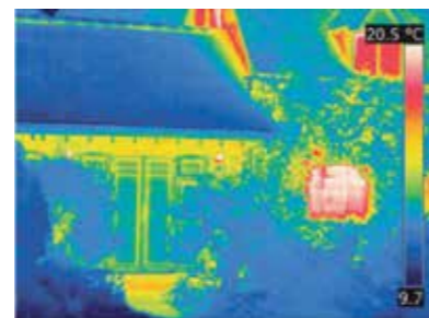
Heat loss from a single glazed window
